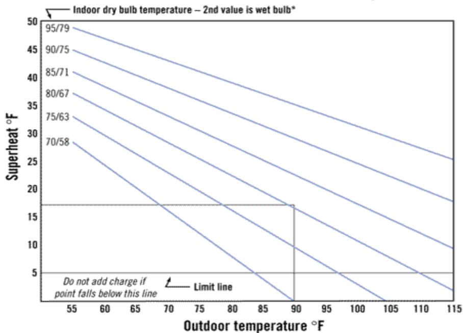
Chart based on 400 cfm/ton indoor air flow and 50% relative humidity.
